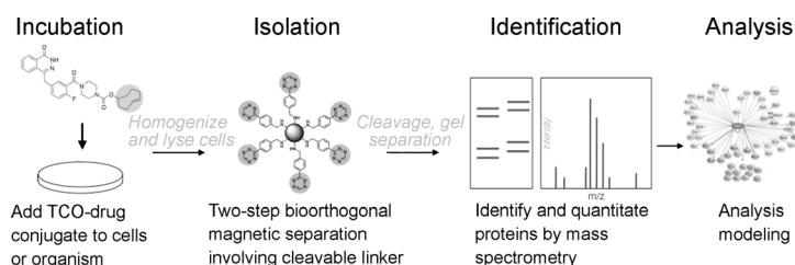
Figure 1. Overview of steps from drug administration to analysis involved in bioorthogonal proteomics. Live cells are incubated with a TCO-drug conjugate. Cell lysates are then prepared and the TCO-drug conjugate bound to the target protein is isolated using a Tz-labeled cleavable linker decorated on streptavidin magnetic beads. The protein is then run on an SDS-PAGE gel, and the desired bands are isolated and submitted for mass spectrometry analysis.
