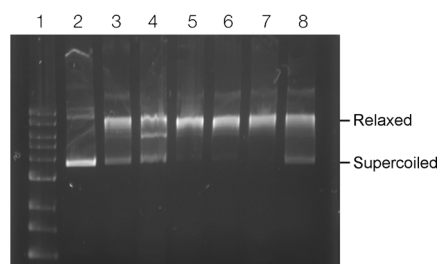
Figure 4. TOP2A DNA relaxation assay. TOP2A was incubated with pAcGFP1 DNA for 30 min at 37°C. The reaction was stopped using SDS and protein was digested by proteinase K. Lanes: 1) 1kb DNA ladder; 2) pAcGFP1 DNA; 3) DNA incubated with TOP2A; 4–8) DNA incubated with TOP2A and 4) 100 \mu M Etoposide; 5) 500 nM Olaparib, 6) 1 \mu M Olaparib; 7) 10 \mu M Olaparib; 8) 100 \mu M Olaparib.
