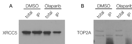
Figure 3. Co-immunoprecipitation (co-IP) in A2780 cells treated with 0.1 % DMSO or 7 \mu M Olaparib for 1 h. Cells were washed twice and incubated for 30 min to remove excess inhibitor. Cells were then lysed and incubated with PARP1 antibody and subsequently with protein A magnetic beads. After washing, protein complexes were eluted from the beads, boiled, and run on a gel. Western blotting was done on 0.1 % XRCC5 and 1 % TOP2A total lysate or on the IP protein using antibodies against XRCC5 (A) or TOP2A (B).
