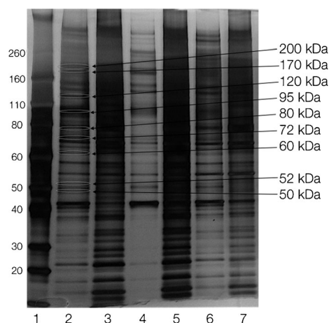
Figure 2. Silver-stained SDS-PAGE gel of the proteomics pull down in A2780 cells. Lanes: 1) marker, 2) Olaparib-TCO, cleaved with 25 mM DT, 3) protein left on beads from (2), 4) Olaparib-TCO, cleaved without DT, 5) protein left on beads from (4), 6) DMSO, cleaved with 25 mM DT, 7) protein left on beads from (6). Sizes on the right indicate bands that were isolated for mass spectrometry analysis.
