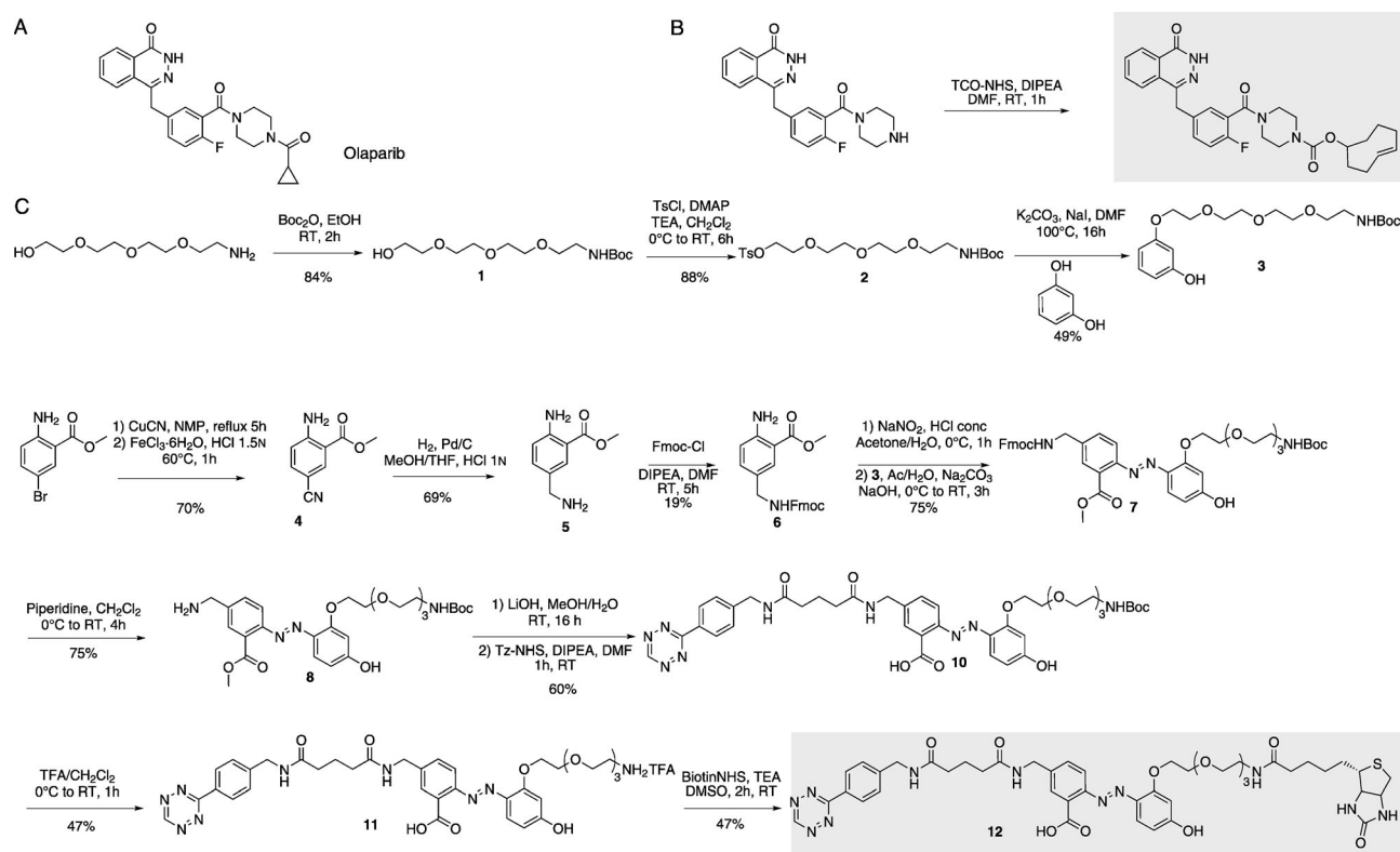
Scheme 1. Synthetic scheme of Olaparib-TCO and the cleavable linker. A) Olaparib for comparison, B) Olaparib-TCO conjugate, and C) cleavable linker. Key components shaded in gray.
